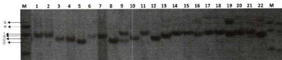
Gambar 2. Produk PCR dengan marka RM105 pada 22 padi lokal Toraja Utara. M = DNA ladder (Promega ΦX174 DNA/HinfI), G = Ukuran alel DNA padi lokal (155,08 bp), H = DNA ladder 151bp, I = DNA ladder 140bp, I1 = Ukuran alel DNA padi lokal (138,53 bp), I2 = Ukuran alel DNA padi lokal (135,11 bp), I3 = Ukuran alel DNA padi lokal (130,22 bp). 1 = Pare Loto-loto, 2 = Pare Lotong Tanduk, 3 = Pare Pulu Lotong, 4 = Pare Pulu Mandoti, 5 = Pare Cina, 6 = Pare Tallang, 7 = Pare Lea, 8 = Pare Seko, 9 = Pare Mansur Buri, 10 = Pare Pulu Kombong, 11 = Pare Pulu Seba, 12 = Pare Ko'Bo, 13 = Pare Birri, 14 = Pare Ambo, 15 = Pare Pulu Lalodo, 16 = Pare Mansur Putih, 17 = Pare Mansur Putih, 18 = Pare Mandi, 19 = Pare Barri Rarang, 20 = Pare Jawa, 21 = Pare Pulu Kalloko, 22 = Pare Barri Busa
